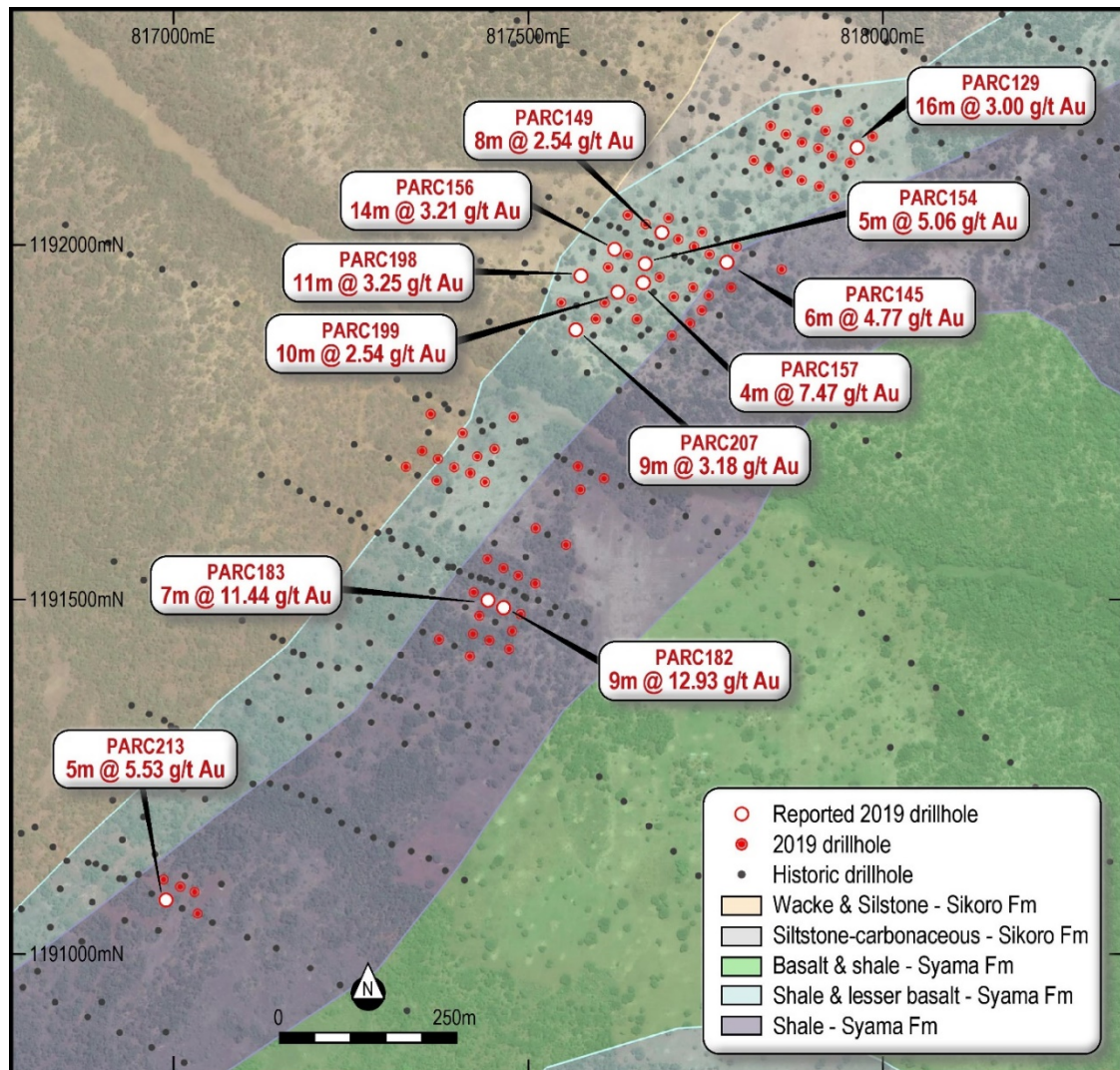
Figure 4: Paysans drill hole locations over geology and satellite imagery
