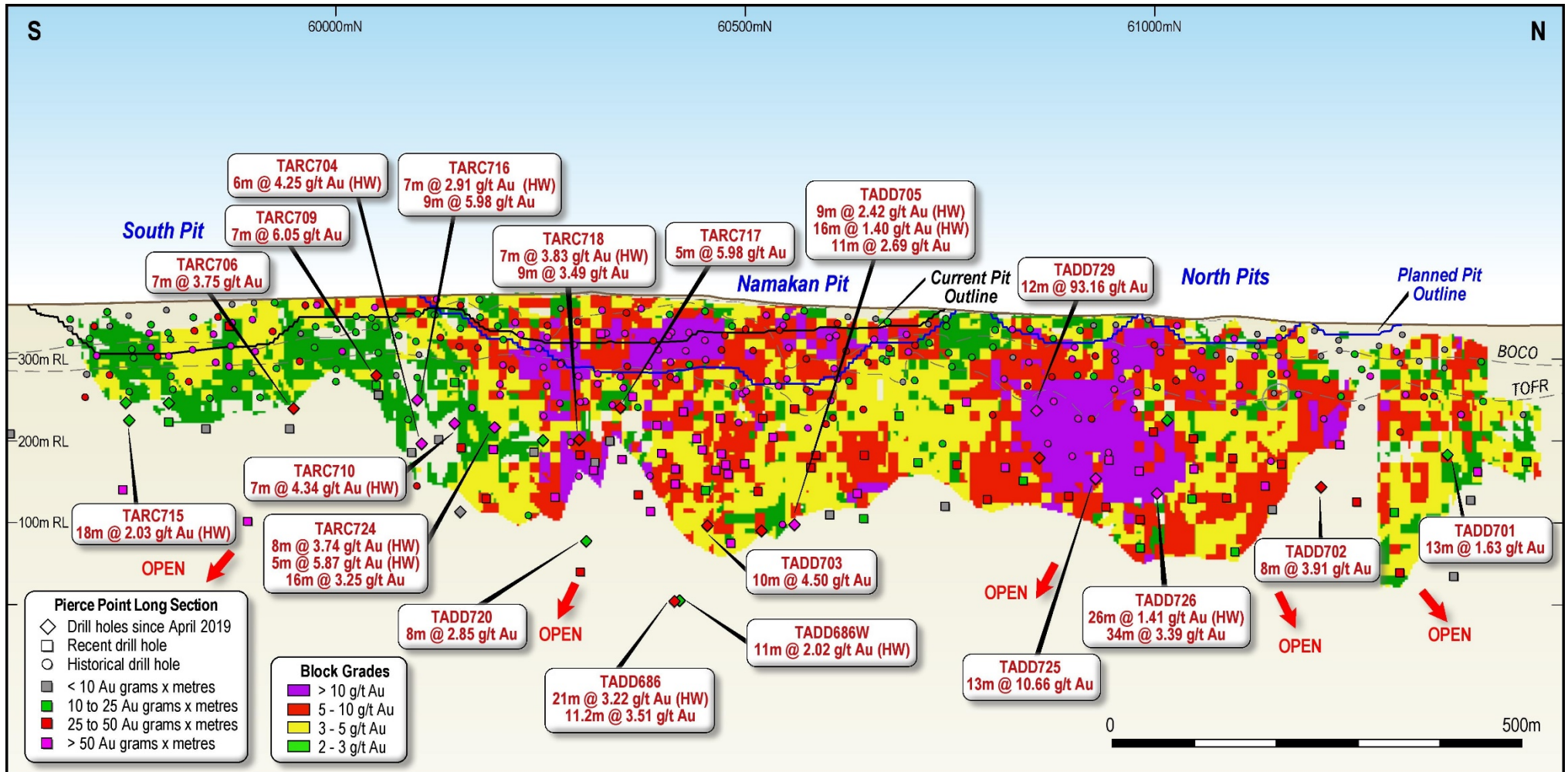
Figure 2: Tabakoroni Longitudinal Section with Resource Model and drillhole pierce points
