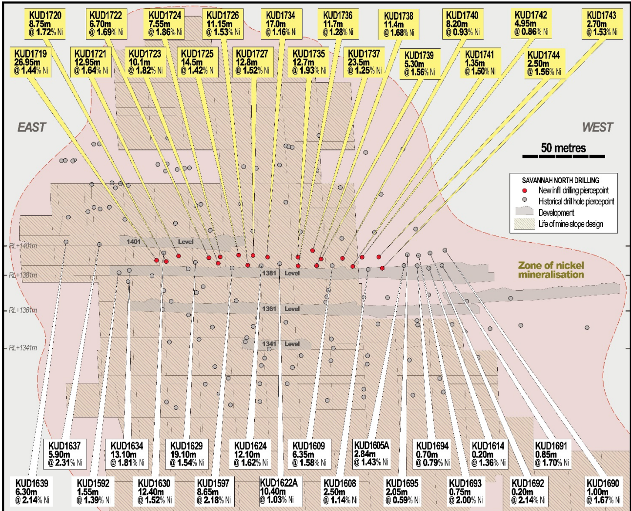
Figure 1: Long-section of the 1381 Grade control and historic drilling intercepts with development drives, proposed slope and mineralisation shapes.
