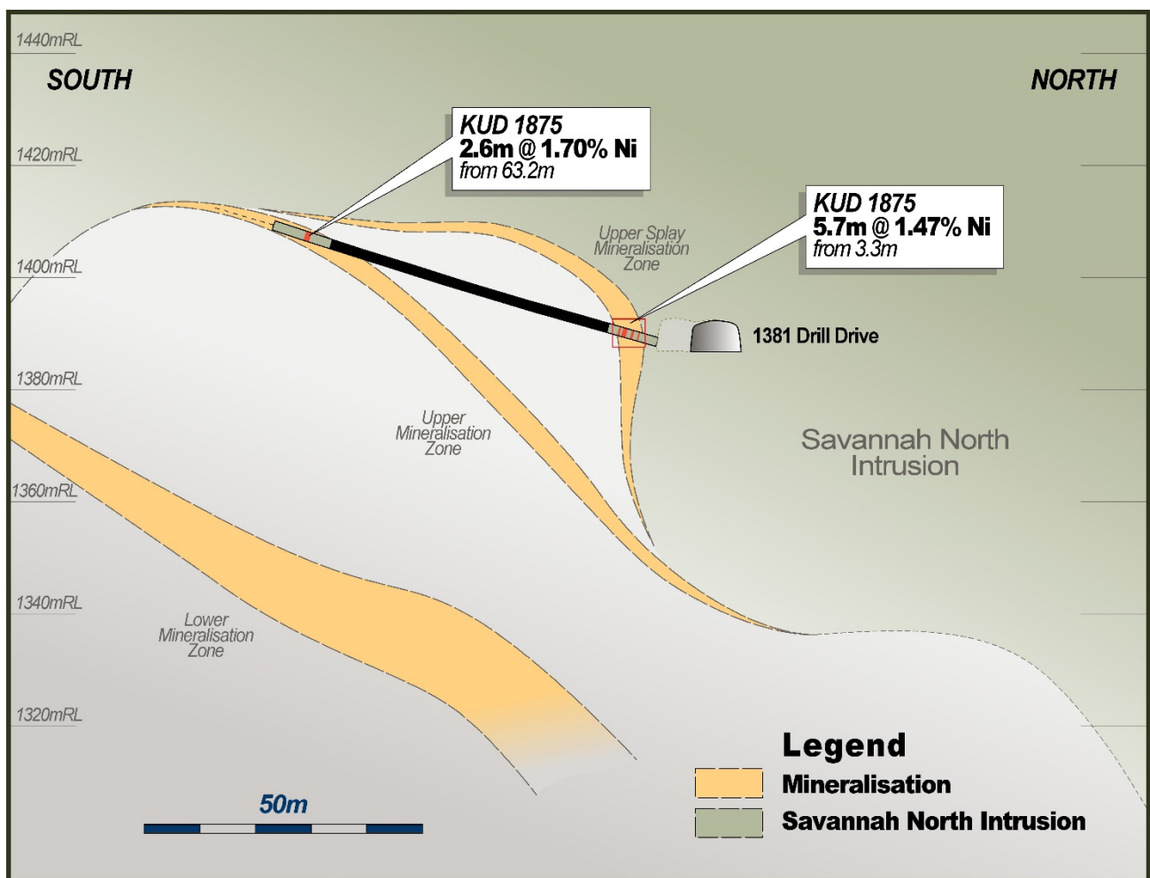
Figure 1: Oblique cross section at approximately 6200mE orientated 015 degrees grid showing drill hole KUD1875 trace and proposed mineralisation model
