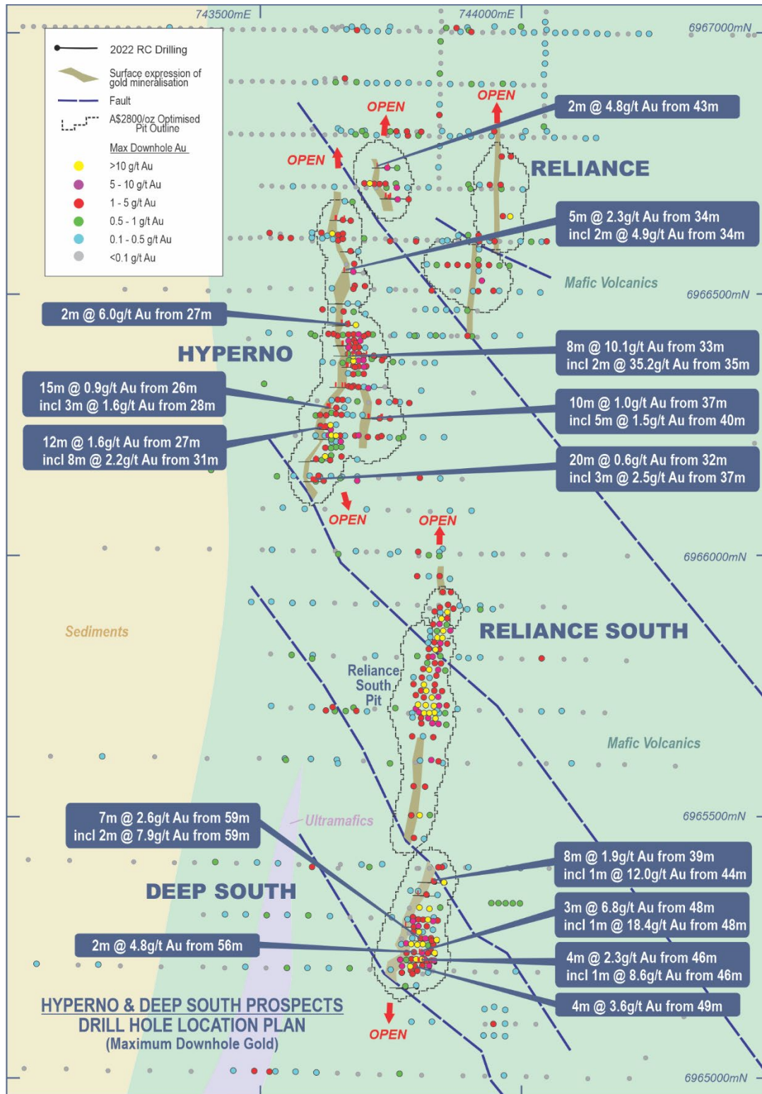
Figure 10: Reliance, Hyperno, Reliance South and Deep South prospects drill hole collar plan coloured by maximum downhole gold, 2022 drilling intercepts >9 GxM (labelled), and A$2800/oz optimised pit shell outlines over interpreted geology.
