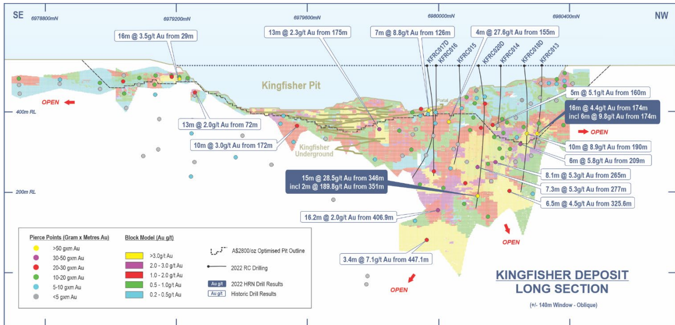
Figure 5: Kingfisher long section (looking SW) showing 2022 drill holes, historic and 2022 gold intercept pierce points coloured by GxM (>24 GxM intercepts labelled), resource block model (coloured by Au) and A$2800/oz optimised pit shell.
