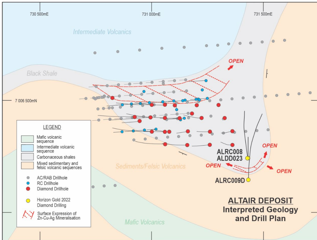
Figure 23: Altair Deposit drill hole location plan showing hole type, drill hole trace and interpreted geology.
