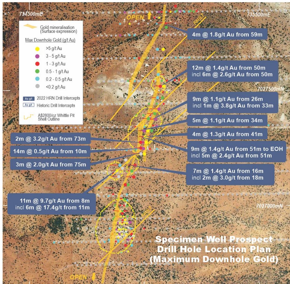
Figure 17: Specimen Well drill hole plan with collars coloured by maximum downhole gold, $2800/oz optimised pit shell outlines, and recent gold intercepts >5 GxM (labelled) over satellite image.
