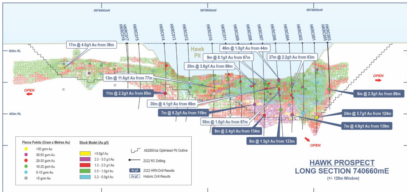
Figure 6: Hawk long section (looking SW) showing 2022 drill traces, historic and 2022 gold intercept pierce points coloured by GxM, current resource block model (coloured by Au) and A$2800/oz optimised pit shell.
